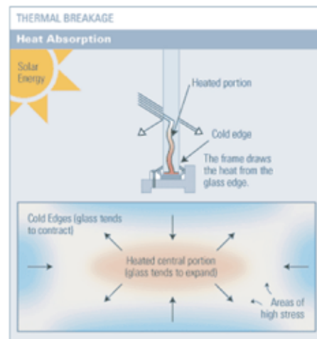
Figure 4 Characteristics of Thermal Breakage.
