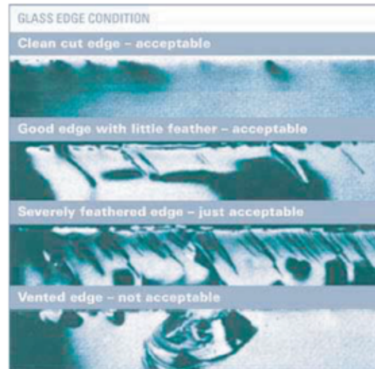
Figure 6 Acceptable Edge of Glass Conditions.
