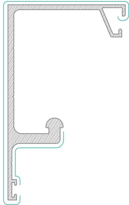
20-PA50TT overhead track AP = 447mm PP = 226mm
