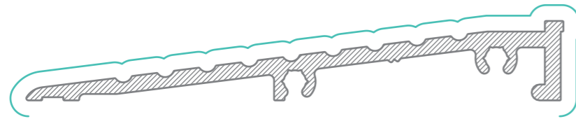
WASF 4013 Ramp Threshold AP = 283mm PP = 136mm
