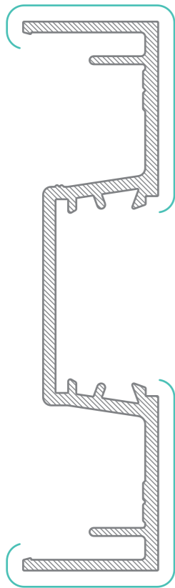
WASF 4207 DG Female Mullion AP = 437mm PP = 115mm
