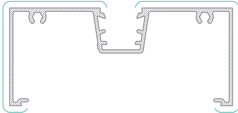
WASF 4008 Light Frame AP = 548mm PP = 183mm
