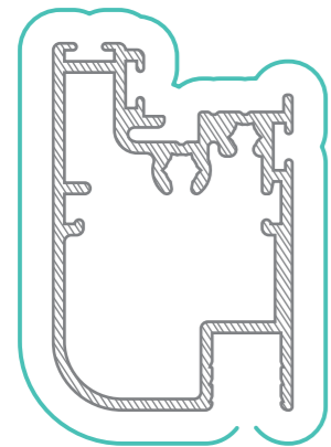
WAAW125 Awning Sash Stile/Rail AP = 200mm PP = 175mm
