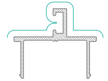
WASF 4211 45mm Door Stop AP = 185mm PP = 77mm
