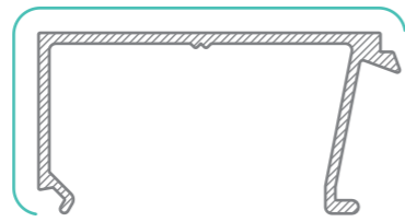
WASF 4002 Still/Transom Bead
