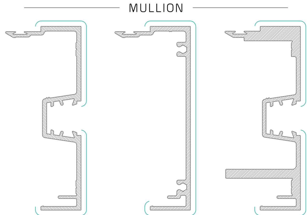
WASF 4006 Self Mating Mullion AP = 456mm PP = 128mm
