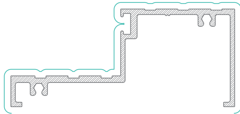
WASF 4025 Open Out Threshold AP = 448mm PP = 206mm
