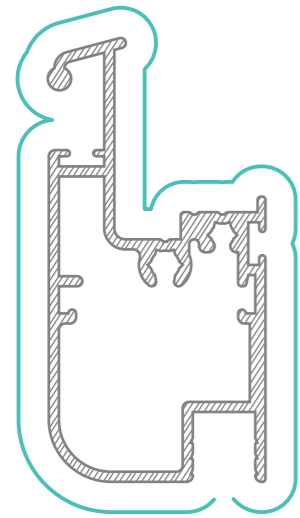
WAAW124 Awning Top Rail AP = 234mm PP = 196mm
