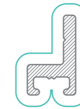
WASF 4020 Door Stop AP = 80mm PP = 44mm
