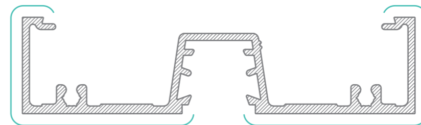
WASF 4029 25mm Centre Glaze Frame AP = 468mm PP = 144mm
