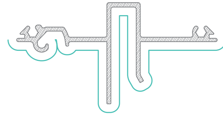
WAAW103 Awning Head Clip-In AP = 406mm PP = 420mm
