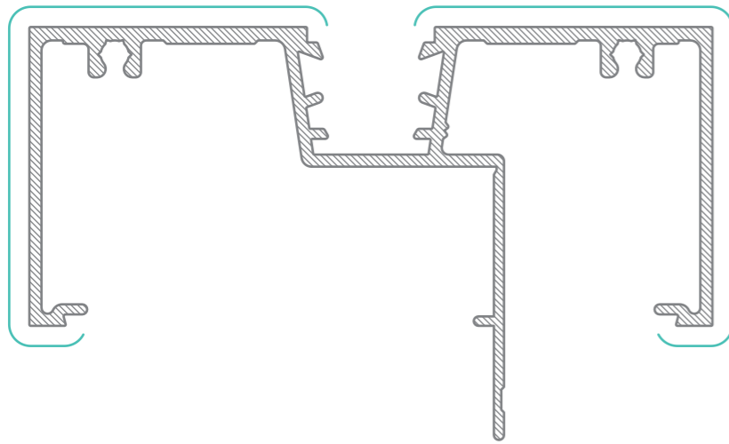
WASF 4018 Frame with Fin AP = 652mm PP = 183mm
