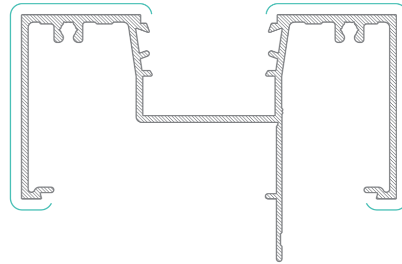
WASF 4218 Frame with Fin AP = 686mm PP = 176mm
