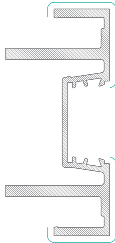
WASF 4209 DG Heavy Male Mullion AP = 573mm PP = 115mm
