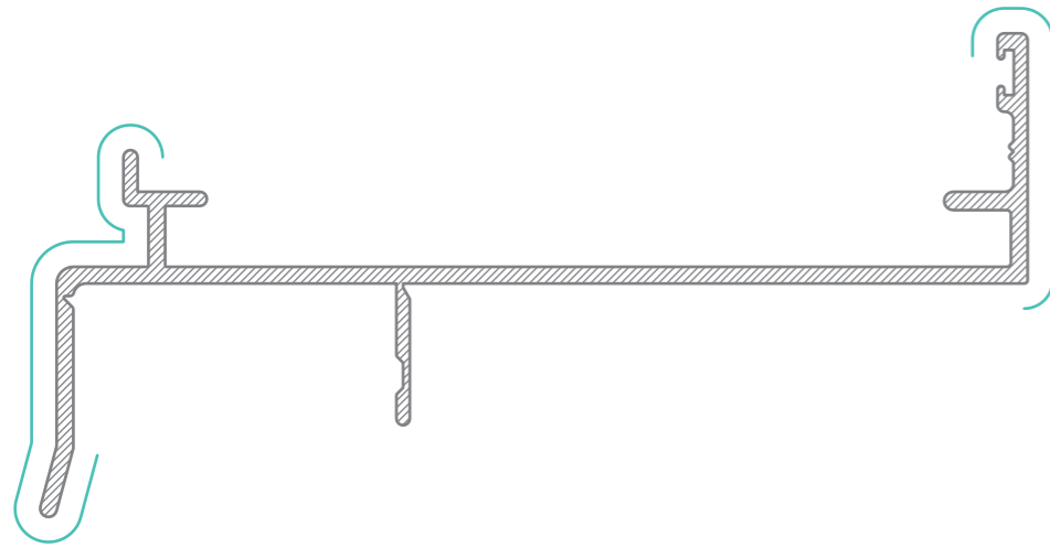
WASF 4024 Subsill with Fixing Fin AP = 450mm PP = 117mm
