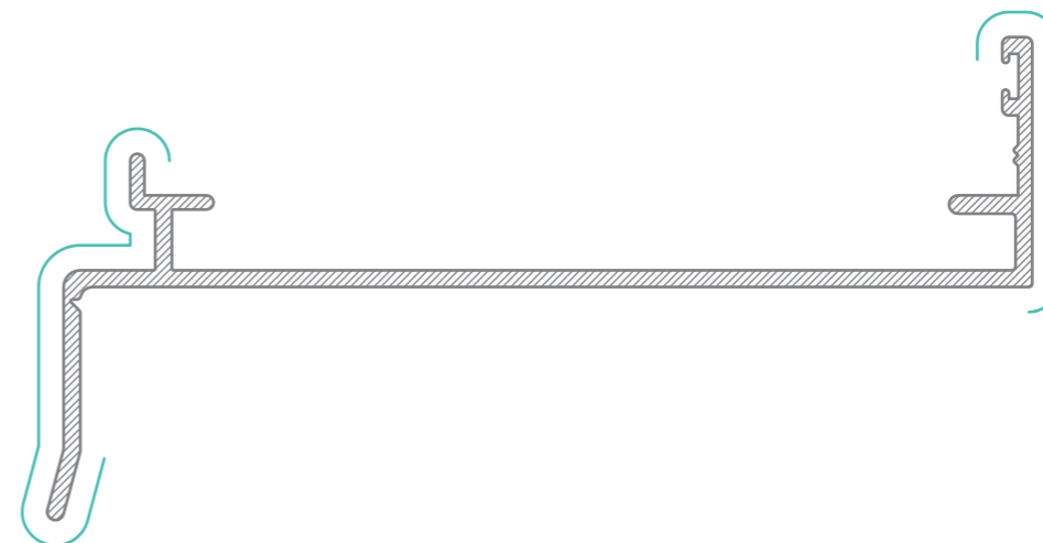
WASF 4014 114mm Subsill AP = 416mm PP = 128mm
