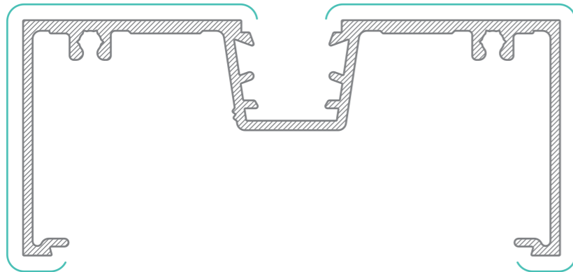
WASF 4000 Frame AP = 546mm PP = 186mm
