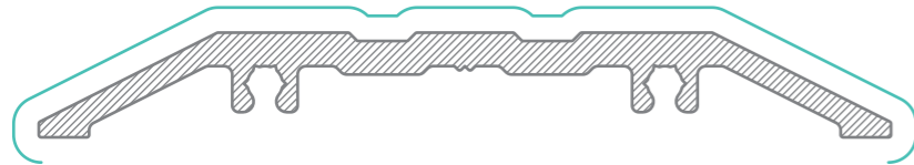
WASF 4023 Concealed Overhead Closer Threshold AP = 263mm PP = 113mm
