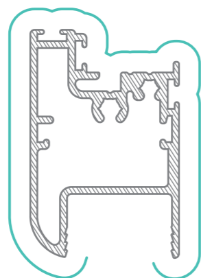
WAAW154 Awning DG Stile/Rail AP = 205mm PP = 162mm
