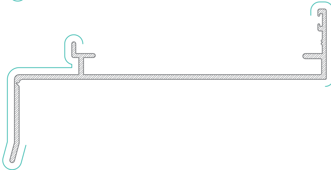
WASF 4015 131mm Subsill AP = 464mm PP = 159mm
