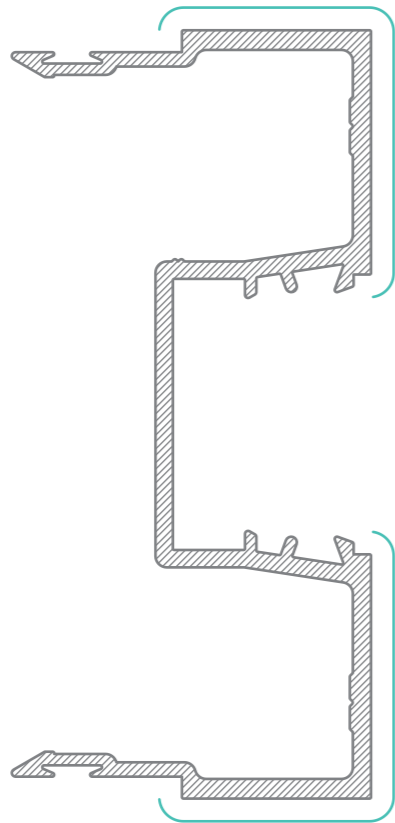
WASF 4206 DG Male Mullion AP = 539mm PP = 115mm
