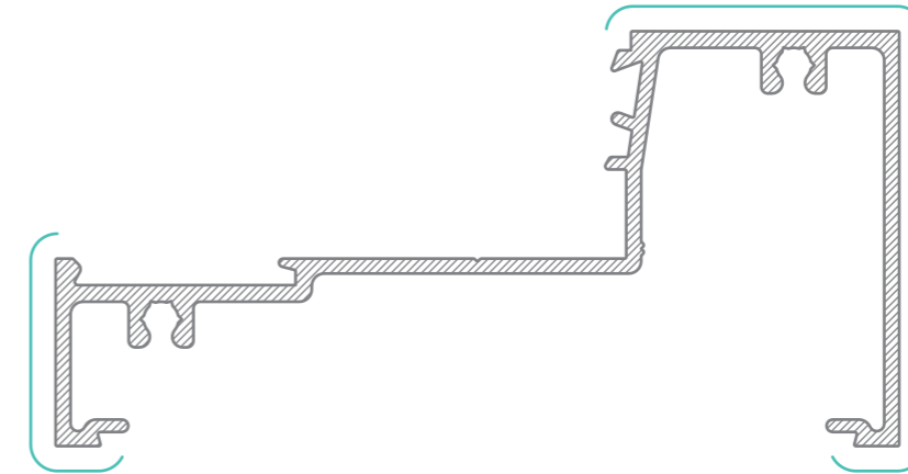
WASF 4201 DG Sill/Transom AP = 491mm PP = 120mm
