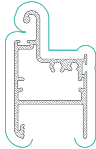
WAAW161 Awning DG Top Rail AP = 248mm PP = 185mm
