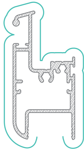
WAAW153 Awning DG Top Rail AP = 240mm PP = 184mm
