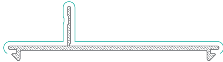
WAWF012 Snap-In Reveal Fin AP = 239mm PP = 126mm
