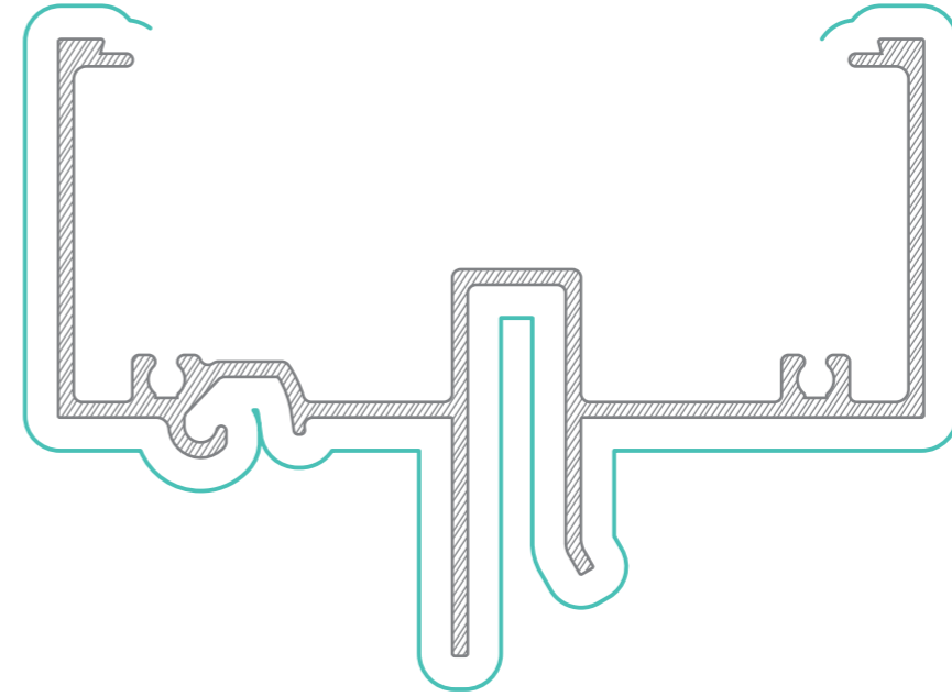
WAAW100 Awning Head AP = 618mm PP = 361mm
