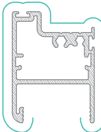
WAAW162 Awning DG Stile/Rail AP = 207mm PP = 144mm
