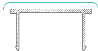
WASF 4205 DG Pocket Filler AP = 146mm PP = 38mm
