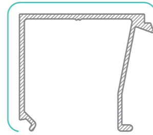
WASF 4202 DG Sill/Transom Bead
