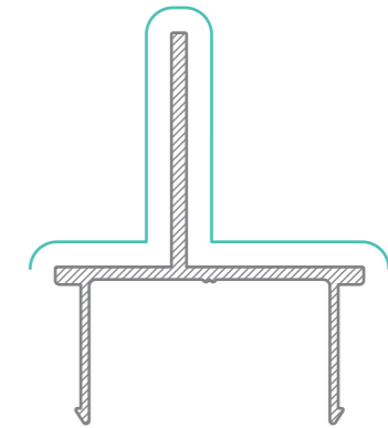
WASF 4210 DG Sash Adaptor AP = 202mm PP = 93mm
