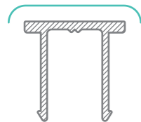
WASF 4005 Pocket Filler AP = 110mm PP = 20mm
