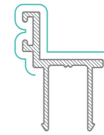
WASF 4026 35mm Door Stop with Mohair AP = 148mm PP = 60mm
