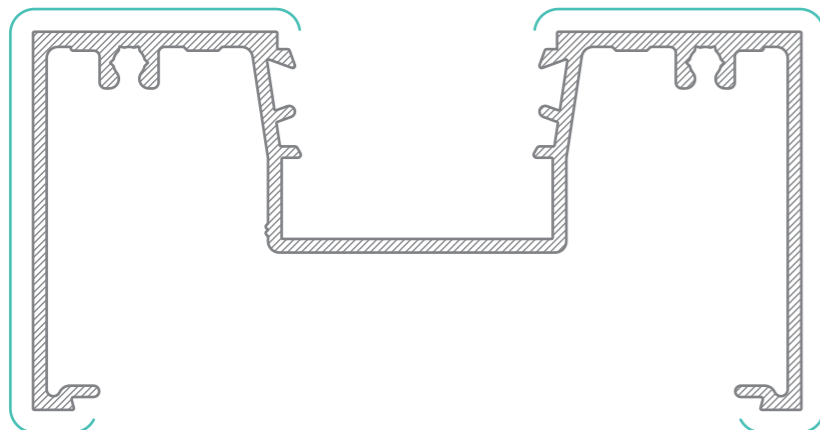
WASF 4200 DG Frame AP = 604mm PP = 176mm
