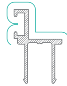
WASF 4009 35mm Door Stop AP = 152mm PP = 44mm
